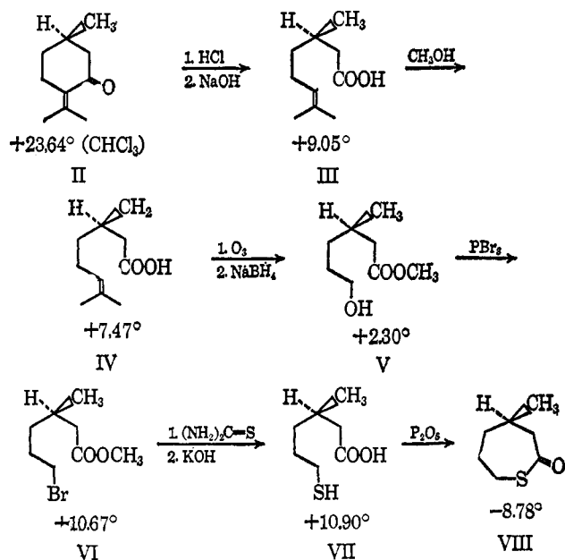
Figure 1. Synthesis of ( R )-(-)-4-methylthiepan-2-one (VIII). Unless otherwise indicated, the specific rotations [\alpha]^{25\text{D}} were measured in methanol.
