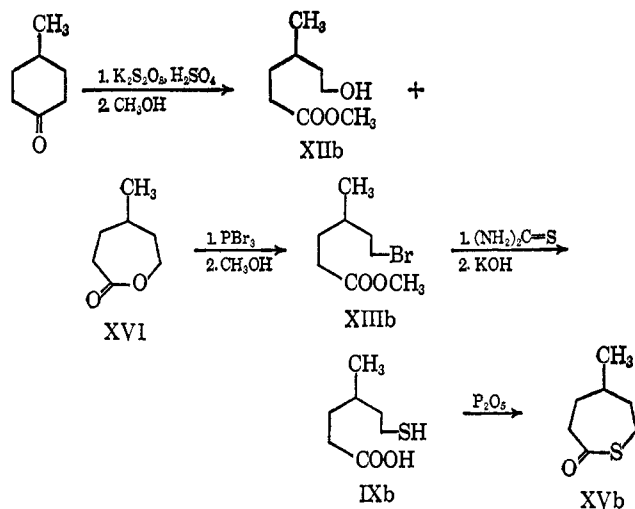
Figure 3. Synthesis of racemic 5-methylthiepan-2-one (XVb).
