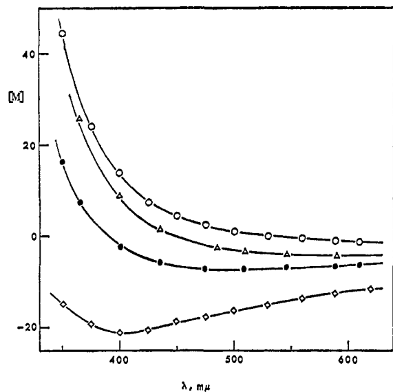
Figure 6. Optical rotatory dispersion of ( R )-(-)-4-methylthiepan-2-one (VIII) in dioxane (○), chloroform (△), tetrahydrofuran (●), and methanol (◇), as measured by Rudolph spectropolarimeter.
