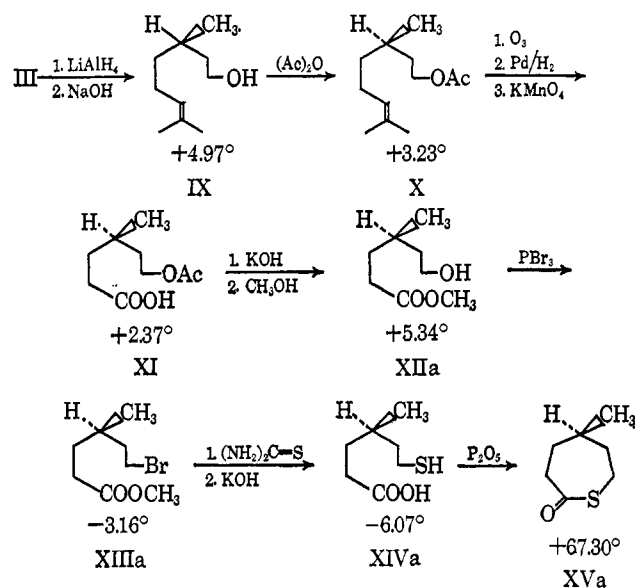
Figure 2. Synthesis of ( R )-(+)-5-methylthiepan-2-one (XVa). The specific rotations [\alpha]^{25\text{D}} were measured in methanol.
